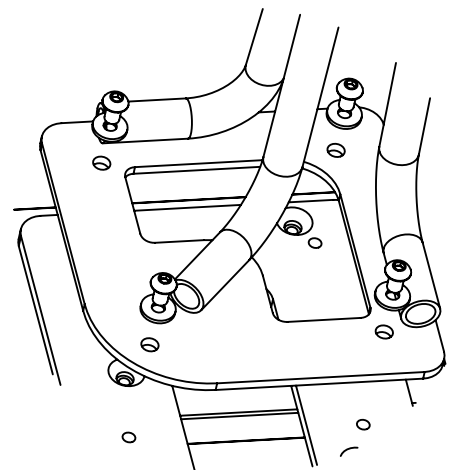
DETAIL J SCALE 1 : 3
