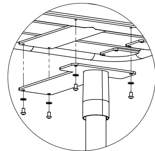
DETAIL C 1:5
