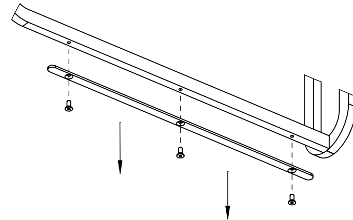
DETAIL F SCALE 1 : 5
