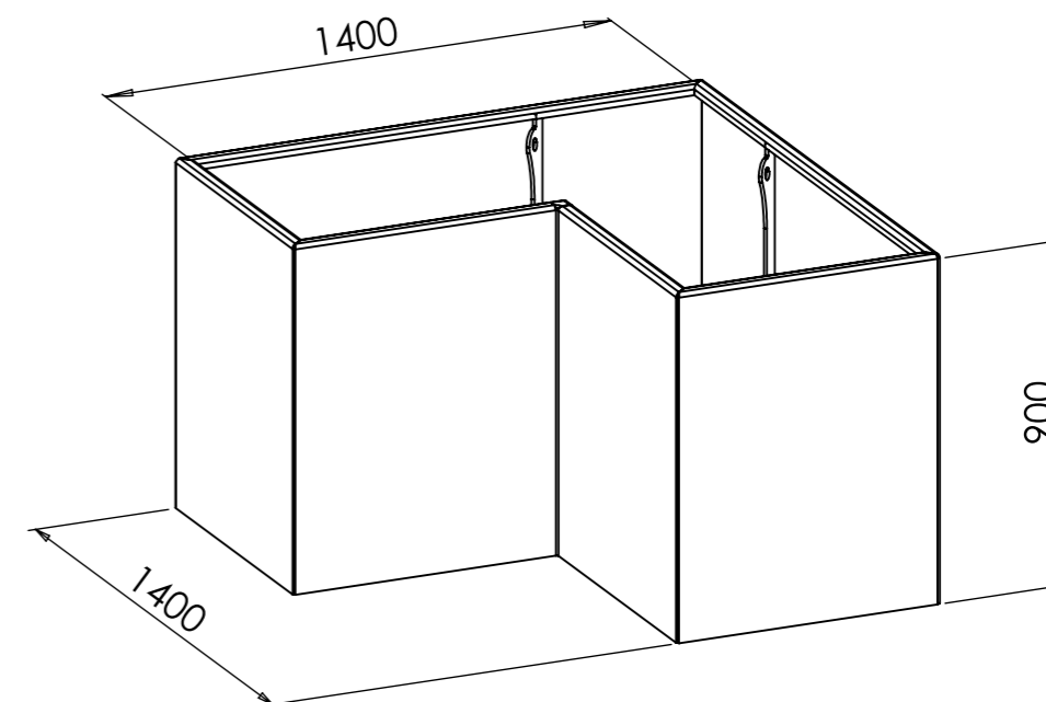
Ö16-76 Angle Planteringskärl, 1000 Liter.
