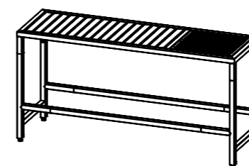
U80-82 Join Bench 650
